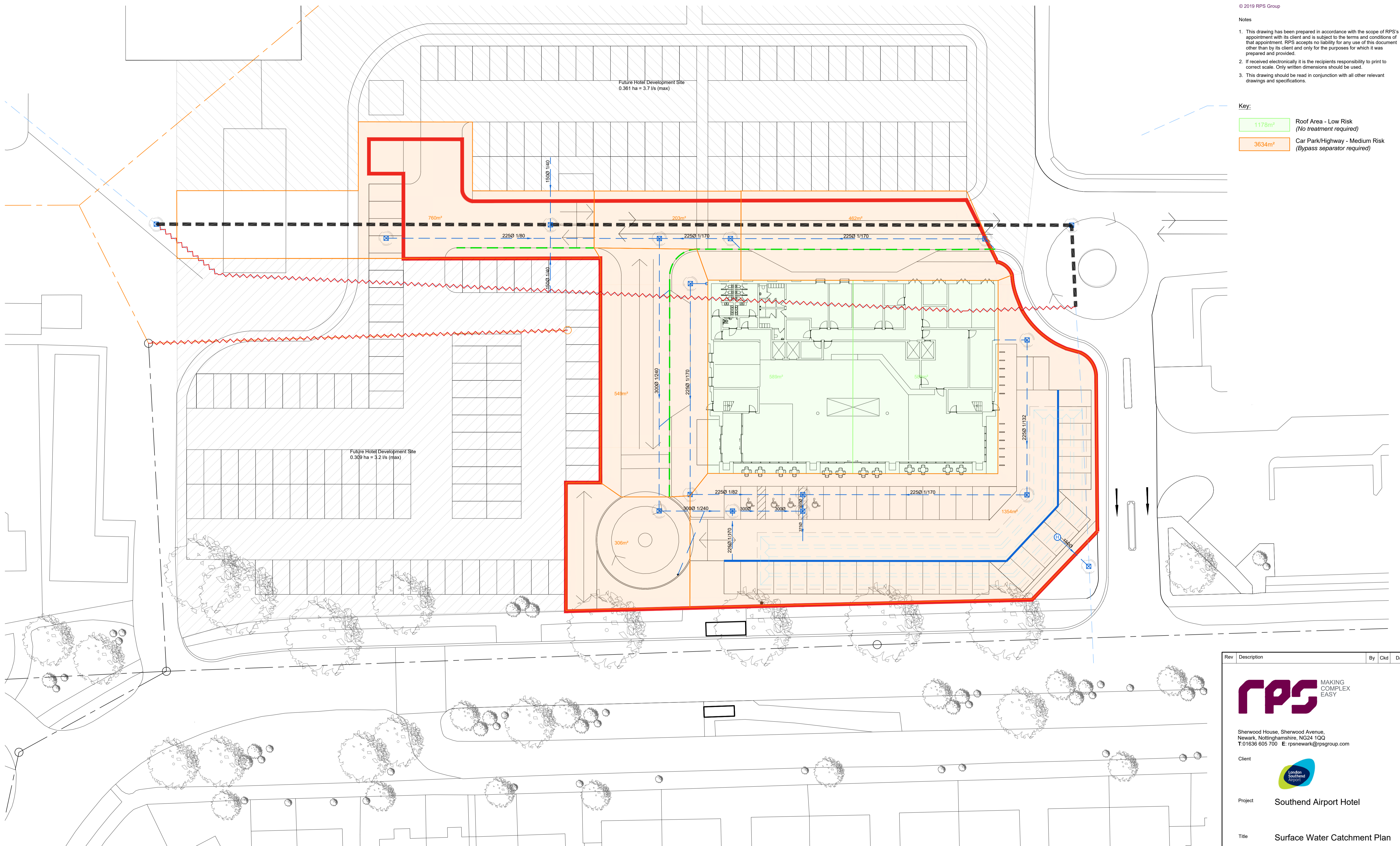
Surface Water Catchment Plan Scale 1:250
